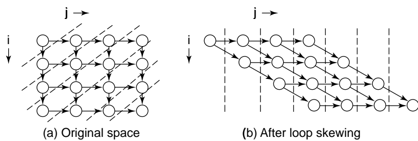
Figure 12.6 Data dependences for Gauss-Seidel iteration.
