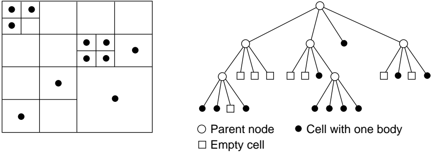
Figure 11.15 Cells and quadtree for a two-dimensional space.
