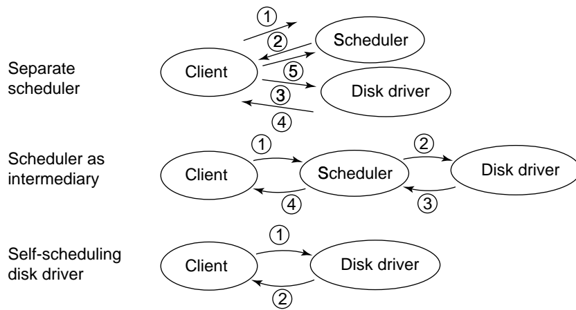
Figure 7.8 Disk scheduling structures with message passing.
