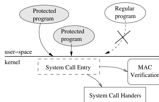
Figure 2. Syscall checking
