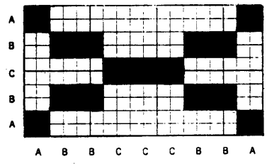
FIGURE 4.3C THREE BLOCK DESIGN Different size blocks Different sequence between threading and treading
