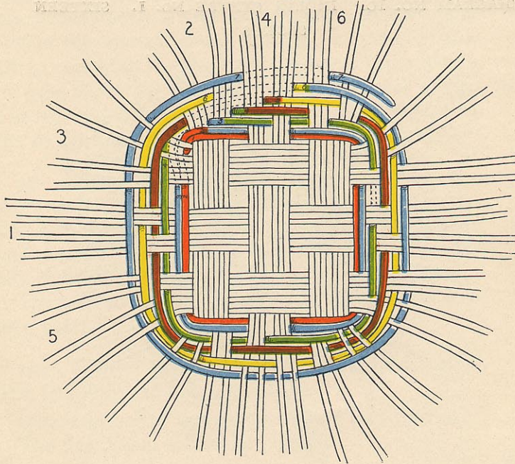
DIAGRAM NO. 19. INDIAN CENTRE NO. 4. TWENTY-FOUR SPOKES
