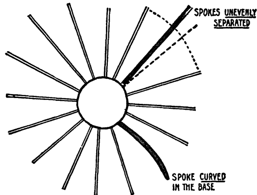
DIAGRAM NO. 21. CORRECT AND INCORRECT BASE SPOKES
