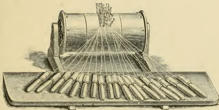
THE VIENNA LACE MACHINE. American Model.
