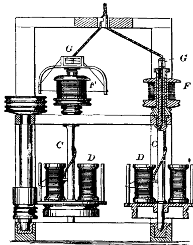
Cord-Covering Machines.
