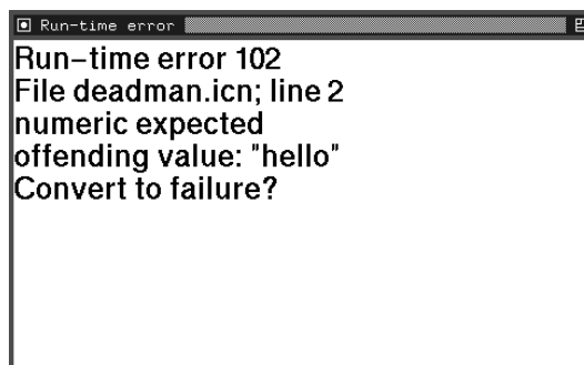
Figure 12.5: Eve's interactive error converter
