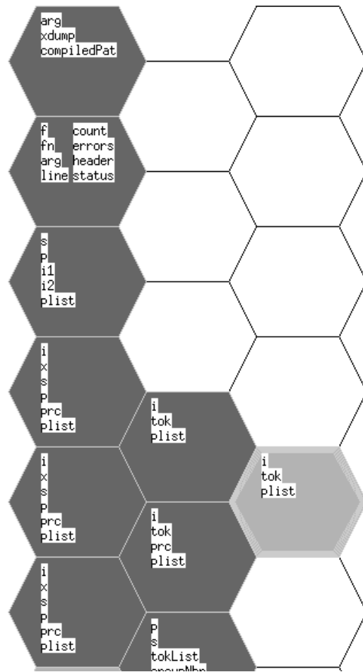
Figure 11.4: Monitoring variables in active procedures
