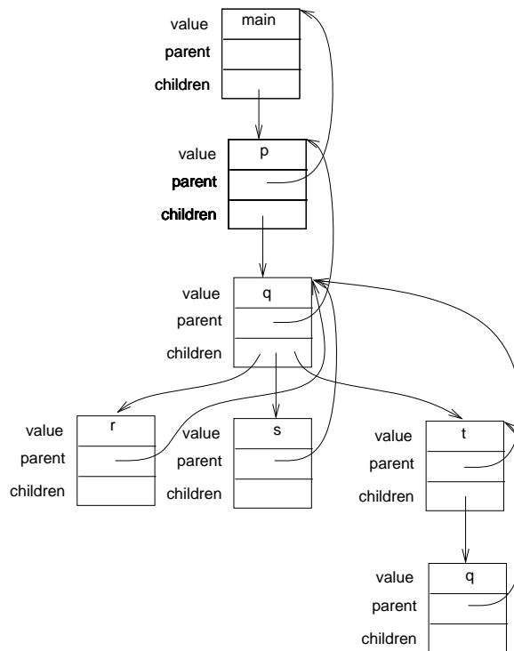
Figure 8.2: An Icon representation of an activation tree
