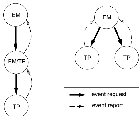
Figure 12.1: Monitoring a monitor; monitoring multiple TPs
