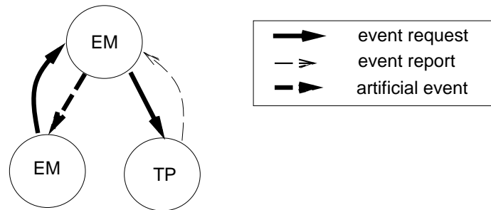
Figure 12.2: Forwarding events to an assistant
