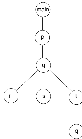
Figure 8.1: An activation tree
