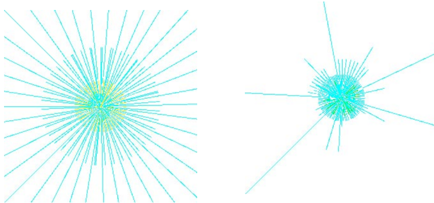
Figure 9.3: Frequent large allocations suggest a problem (left); the program runs twice as fast after a two-line change
